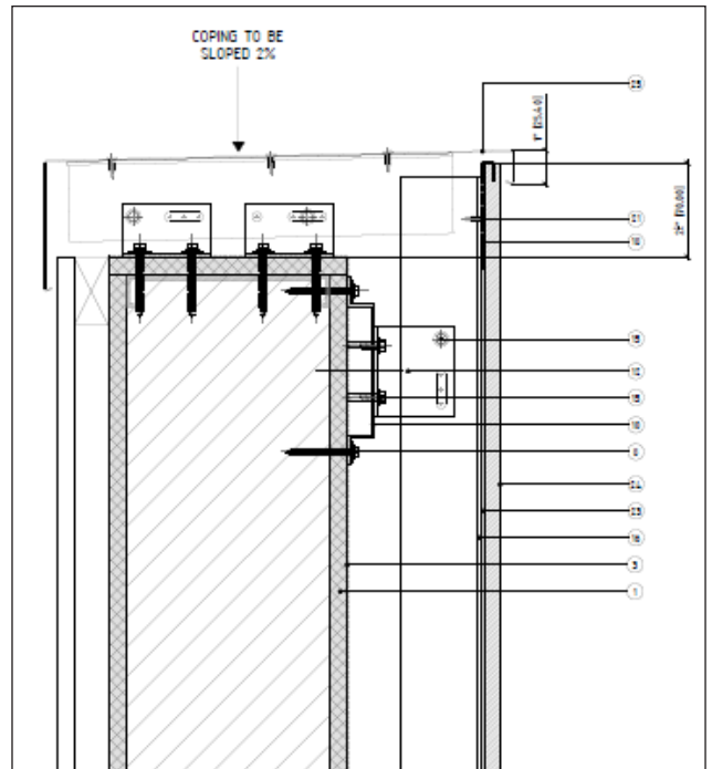
TERMINATION WITH METAL FLASHING/COPING, BY OTHERS
