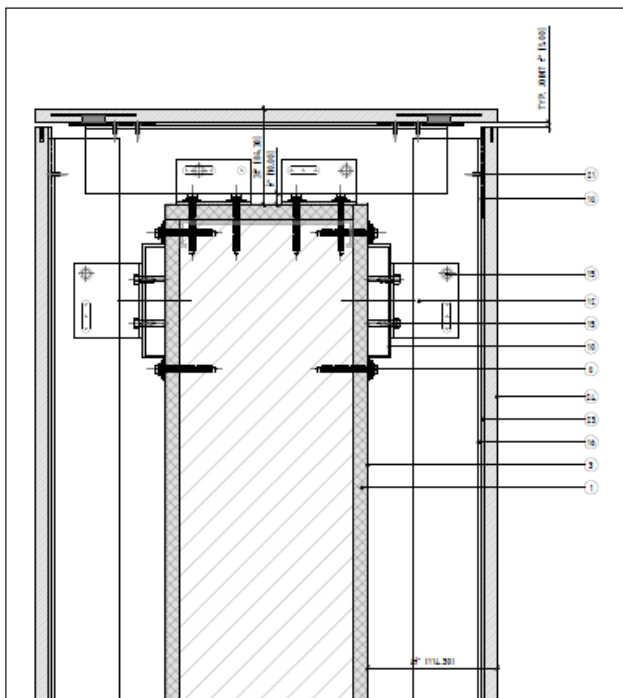
TERMINATION WITH TILE
