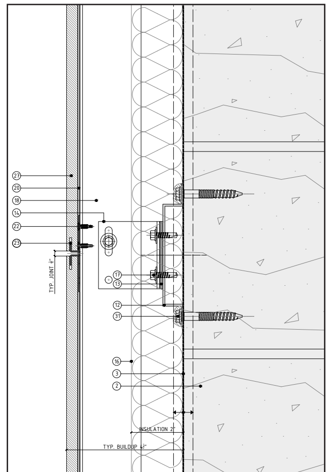
SOLID WALL SECTION EXAMPLE
