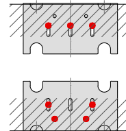
FIGURE 8 - ANCHORING MINIMUM DISTANCE TO EDGE OF WALL
